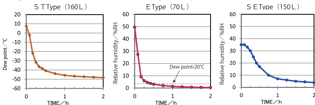
Change in dew point and humidity according to the type of moisture device
